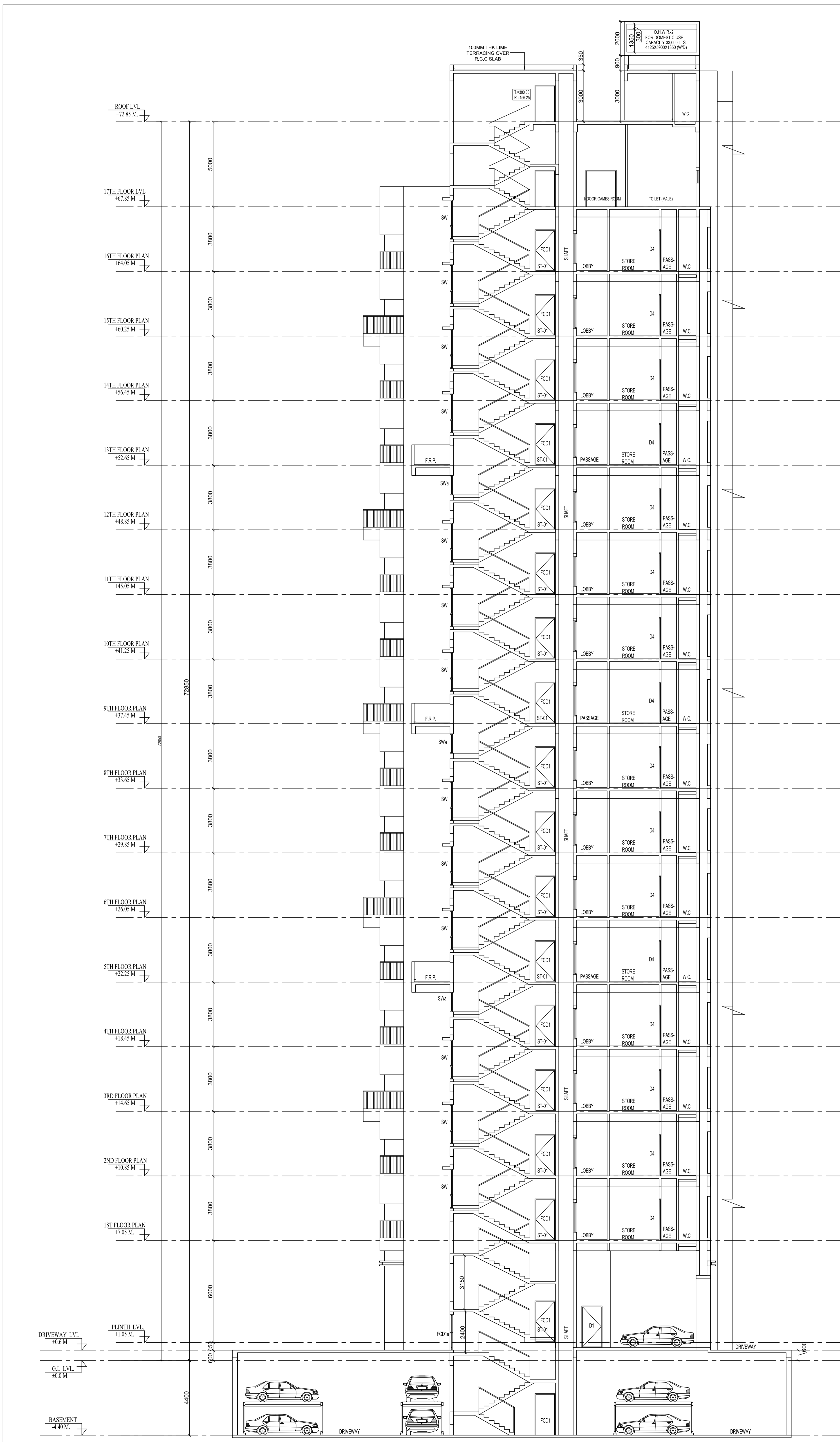
SECTION AT C-C SCALE - 1:100
